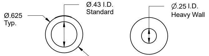
Glass Tube
